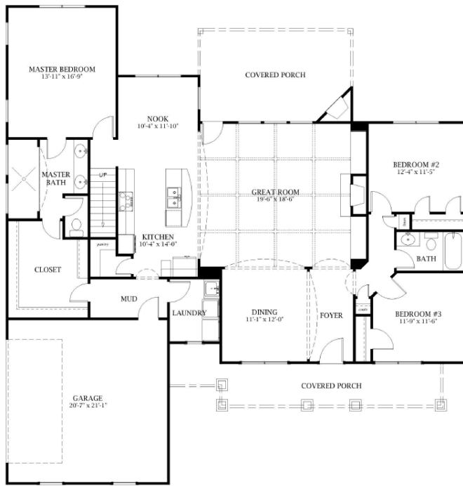
LIVING AREA 2022 sq ft
